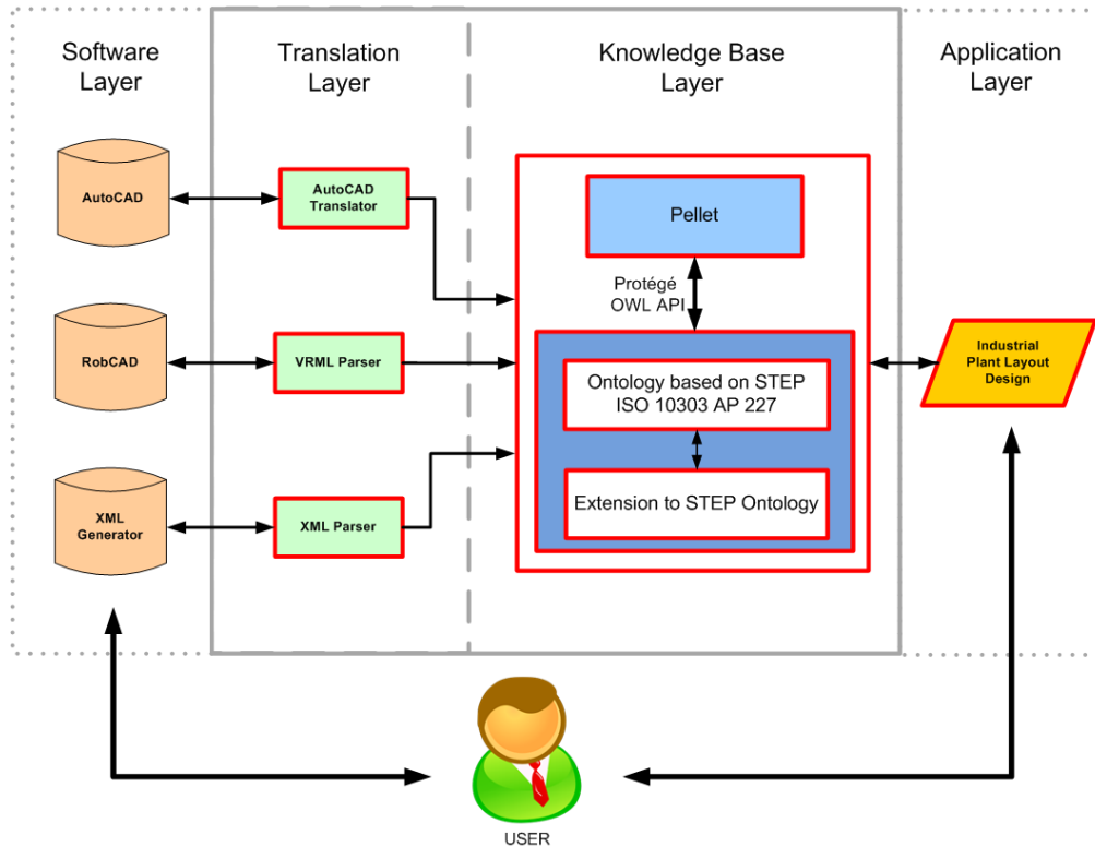
Figure 5. Case study matched in the proposed architecture.
