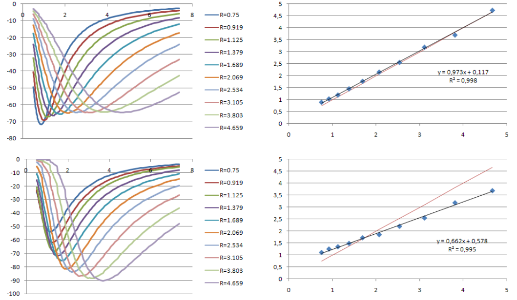
Figure 5.3: Values of the most negative eigenvalue \lambda_3 obtained in the center of the tube for different tube sizes for different Hessian scales \sigma_h and for tubes with Gaussian (top row) and flat convolved (bottom row) section profile. Left column shows all values obtained varying \sigma_h . Right column shows the relationship between the tube radius (x-axis) and radius scale for the maximum values obtained for each radius. Here, the black line shows the obtained linear trend line and the red line represents the line \sigma_h = R .
