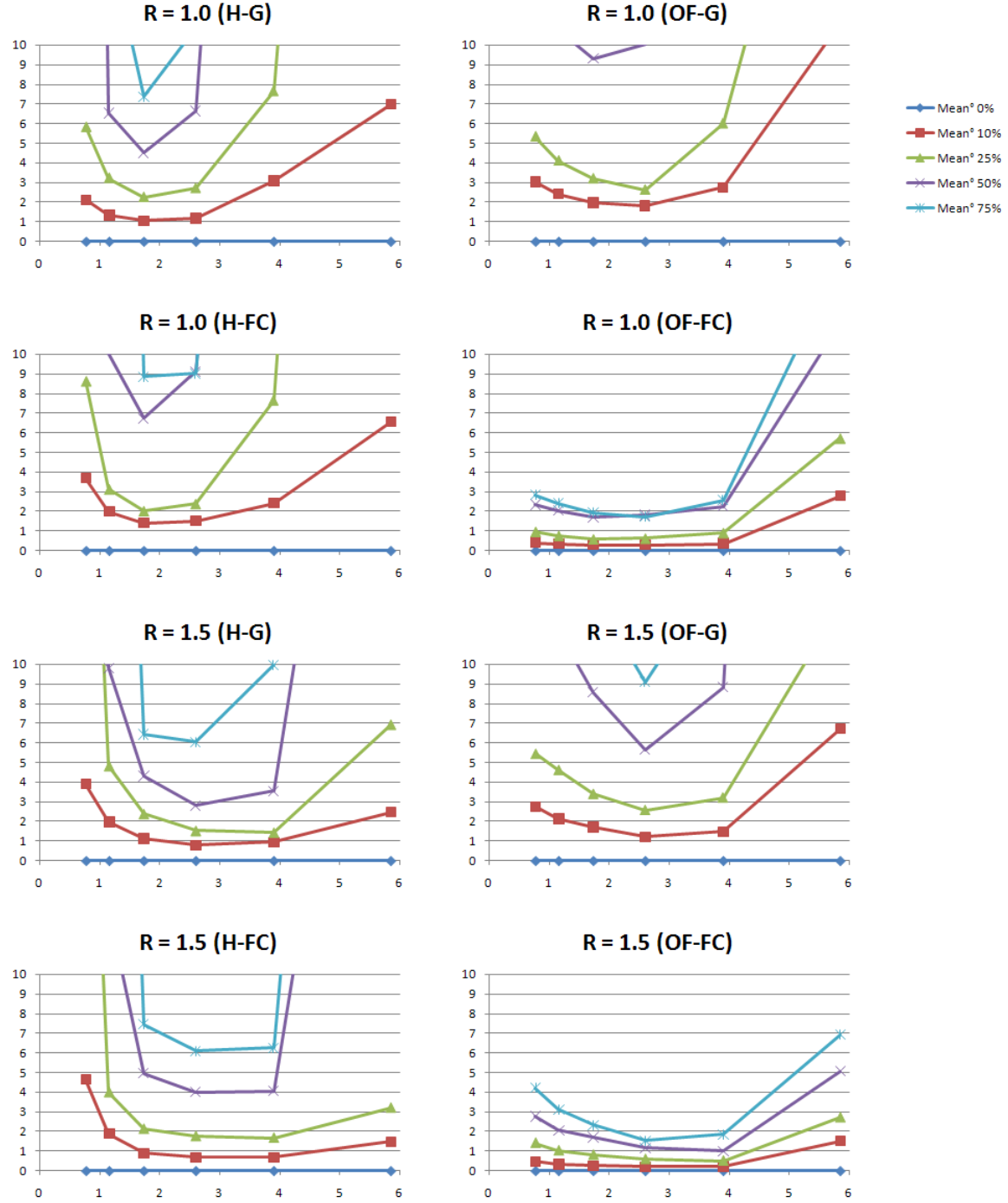
Figure 6.6: Mean values for section angle estimation error (with respect to the z-axis) for different detector scale values (x axis) along tubes of R = 1.0 and R = 1.5 as calculated for the Hessian (H) and Oriented Flux (OF) section estimators and for tubes with Gaussian (G) and Flat Convolved (FC) cross-section. Series show results for different levels of noise with respect to the signal (0, 10, 25, 50 and 75%)
