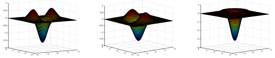
Figure 4.5: Surface plots of \partial^2 g / \partial x^2 (left) and \partial^2 g / \partial y^2 (center) and Laplacian of Gaussian (right). All surfaces are calculated for \sigma = 1.0 .
