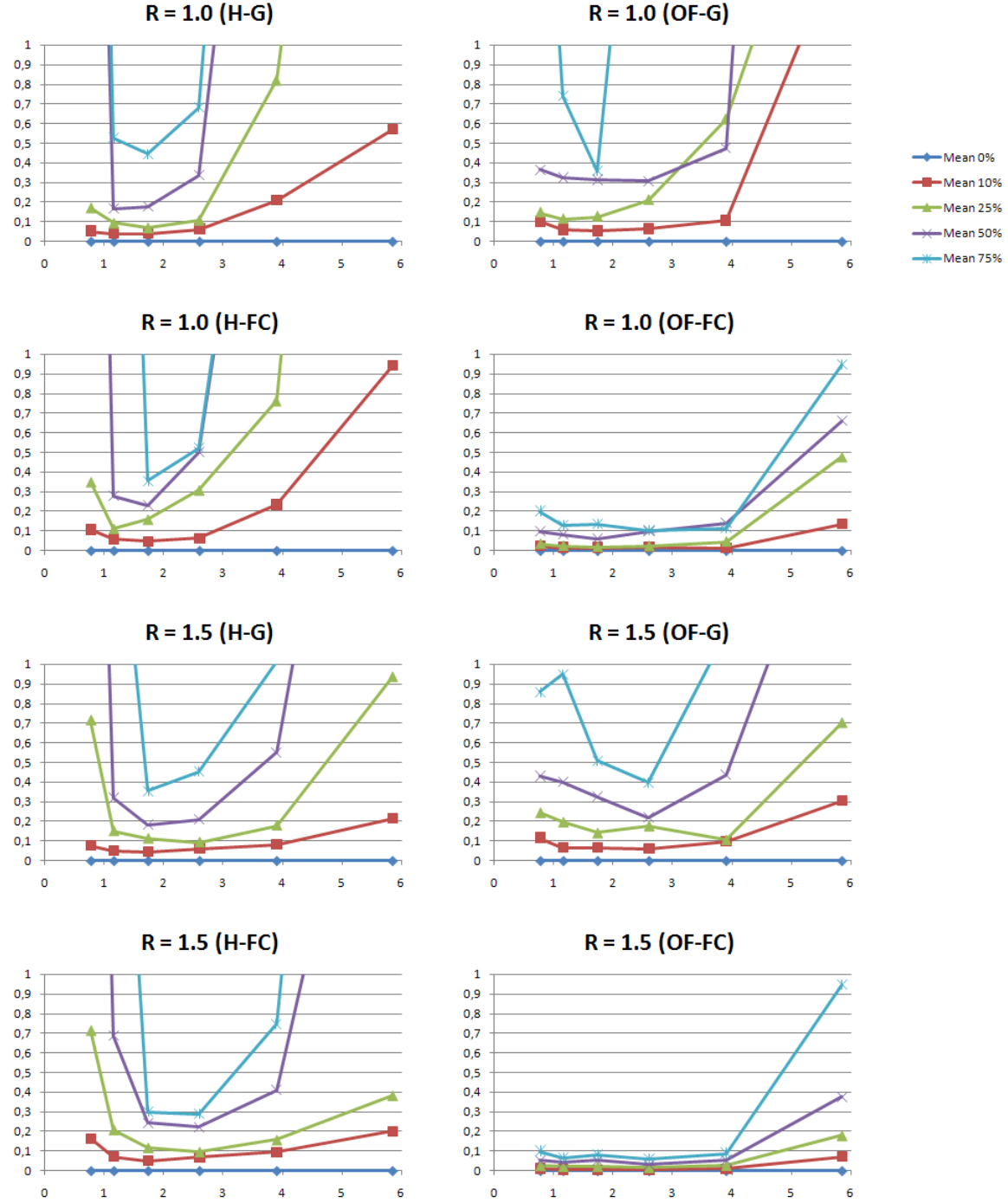
Figure 6.3: Mean values for in-section center point estimation error for different detector scale values (x axis) along tubes of R = 1.0 and R = 1.5 as calculated for the Hessian (H) and Oriented Flux (OF) section estimators and for tubes with Gaussian (G) and Flat Convolved (FC) cross-section. Series show results for different levels of noise with respect to the signal (0, 10, 25, 50 and 75%)
