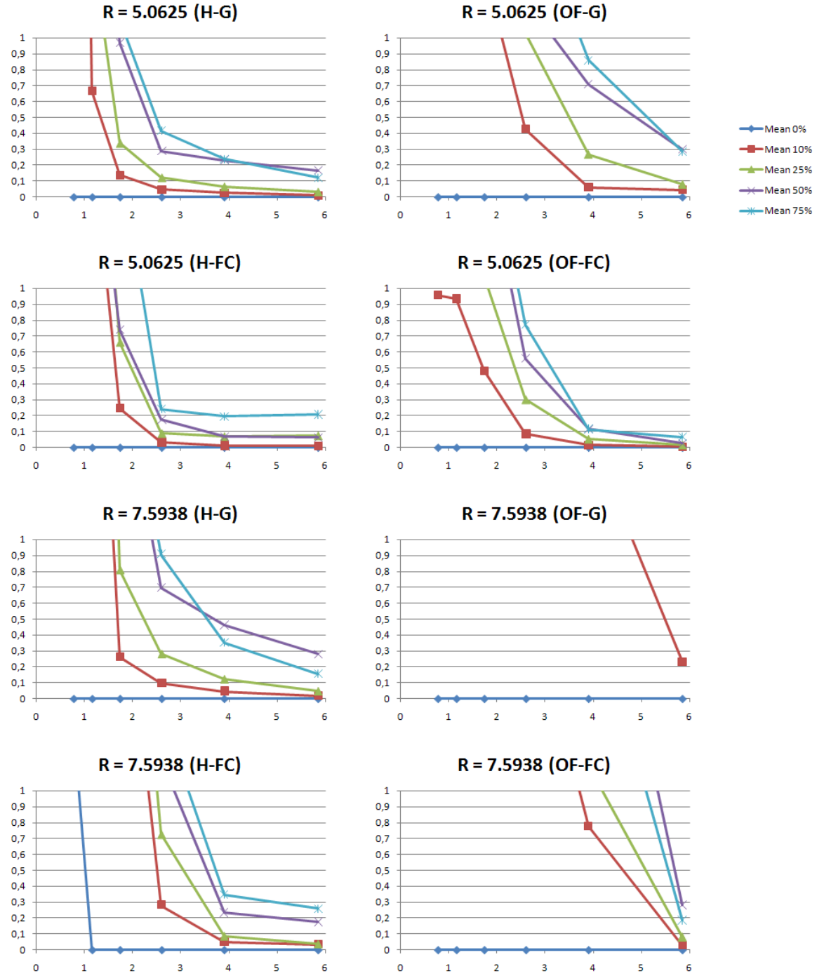
Figure 6.5: Same as Fig. 6.3 for R = 5.0625 and R = 7.5938
