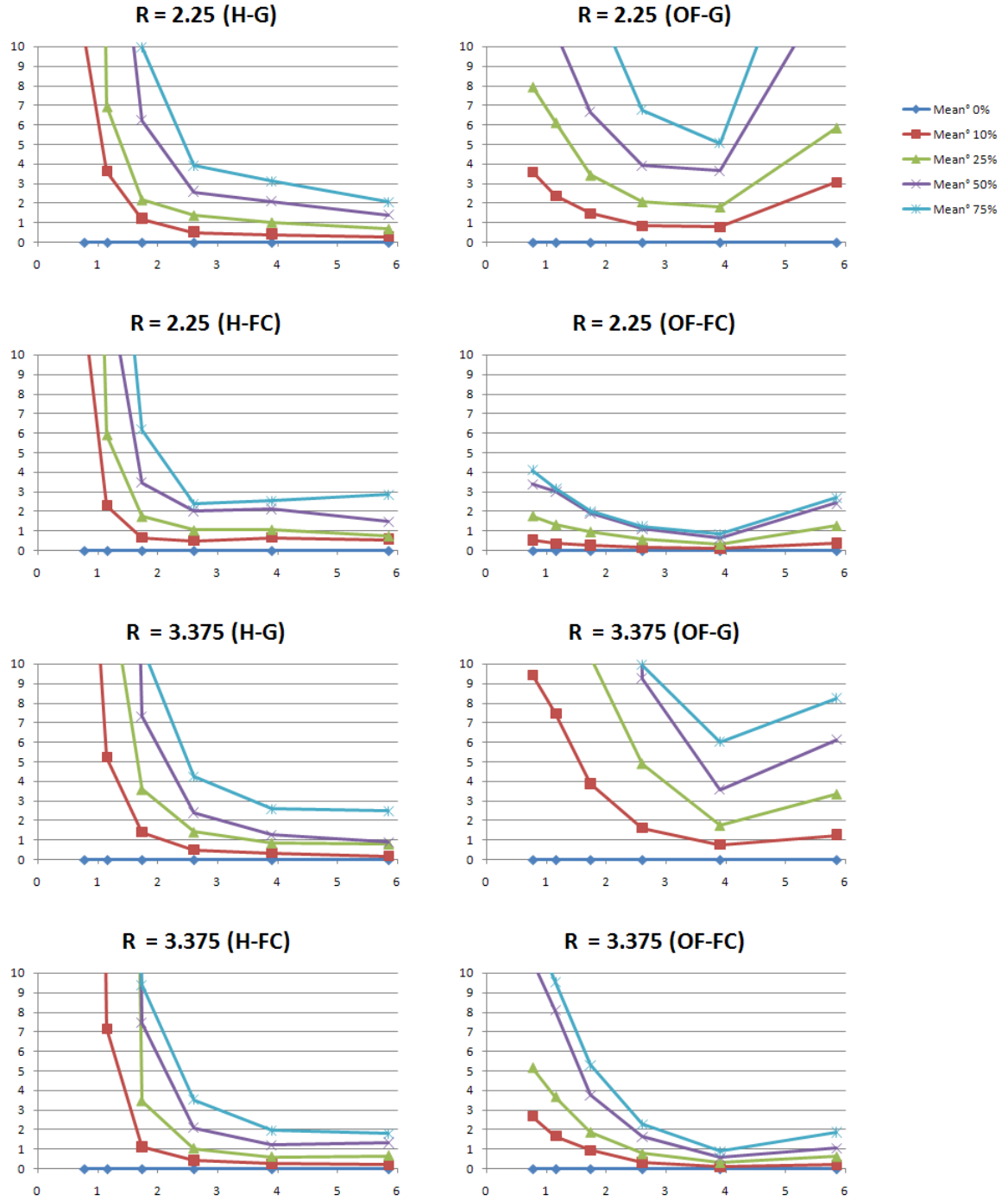
Figure 6.7: Same as Fig. 6.6 for R = 2.25 and R = 3.375
